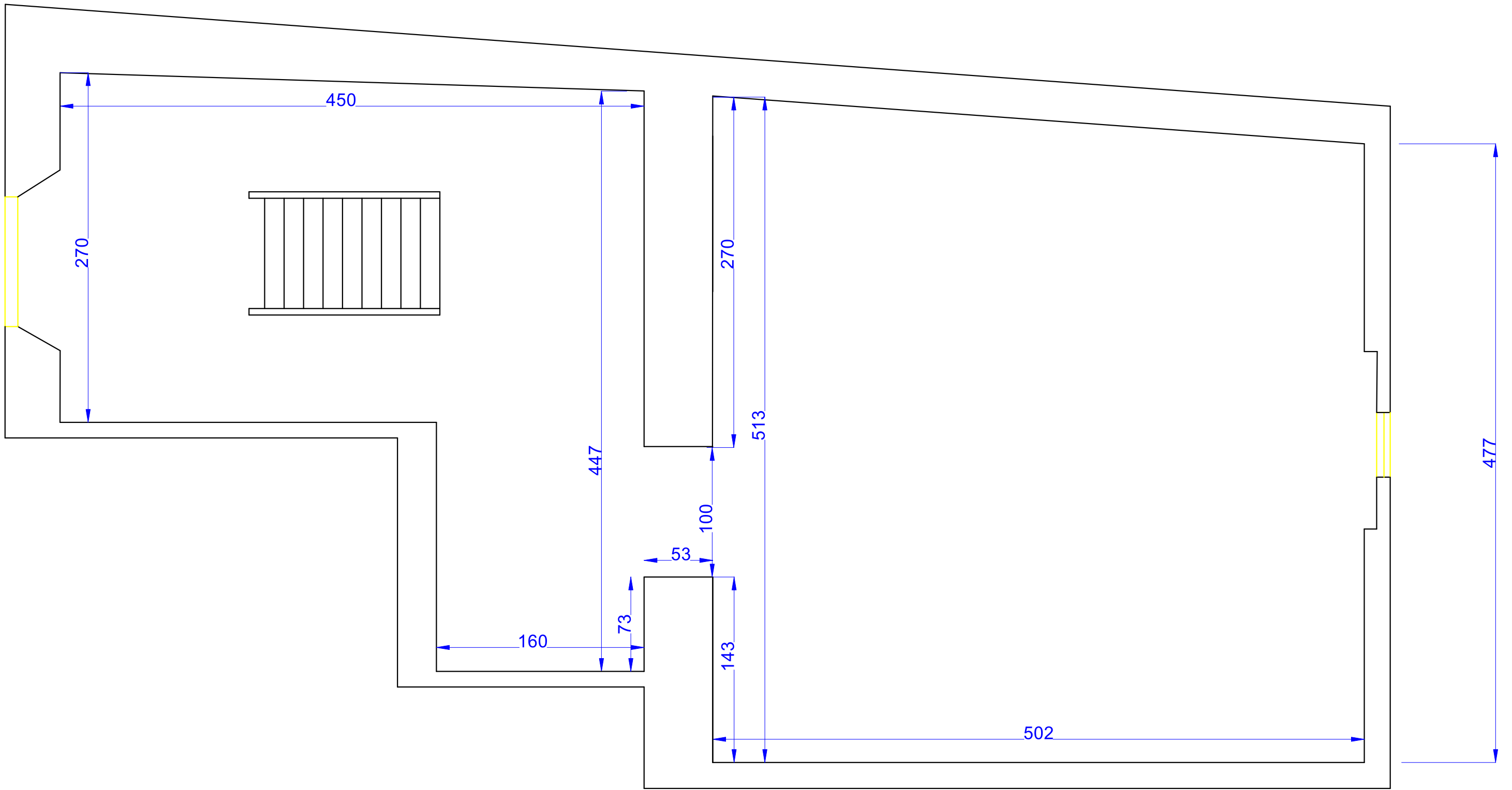
Piano Interrato
